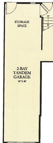
GARAGE LEVEL
